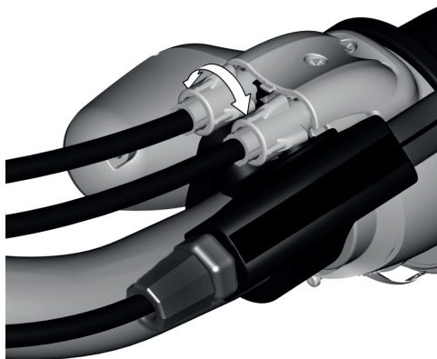
Image 39: Reducing or increasing cable slack by turning the barrel at the grip shifter
