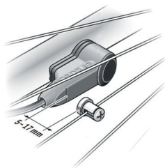
Image 31: Distance between the speed sensor and the speed sensor magnet
