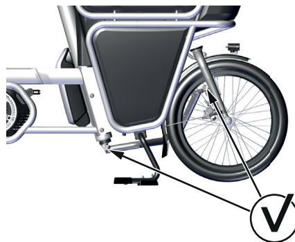
Image 35: Check steering linkage at the ball joints
