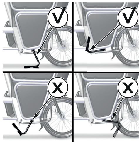
Image 23: Correct and incorrect kickstand positions
