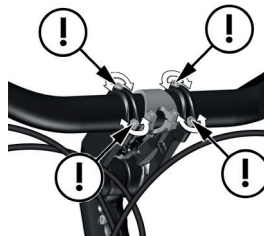
Image 9B: Turning the handlebar angle bolts
