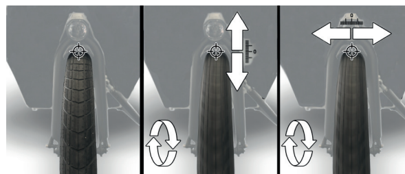
Image 33: Checking the wheel trueness
