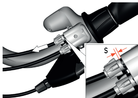
Image 38: Checking cable slack
