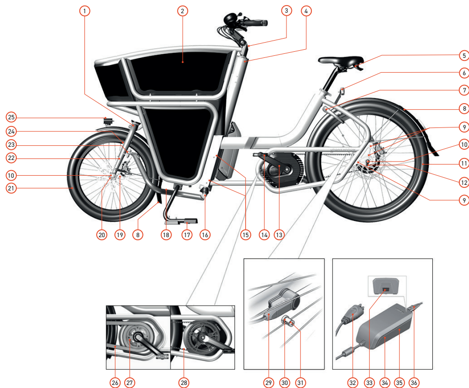
Image 1: General overview (side view)
