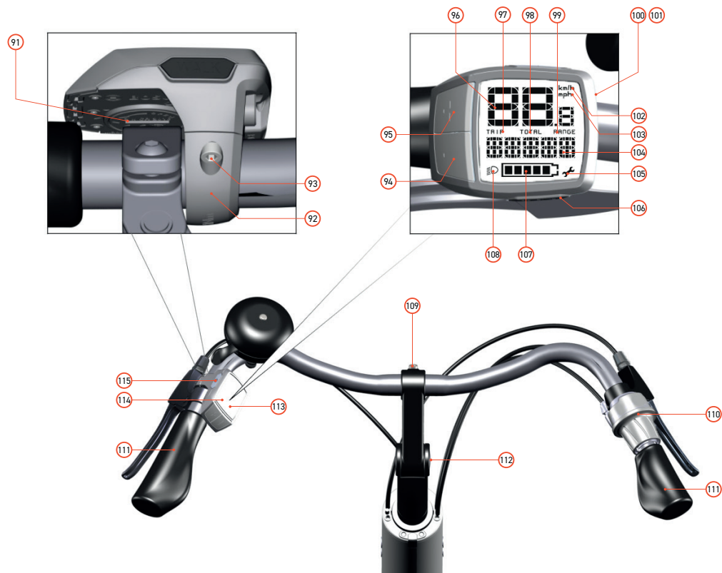
Image 4: Handlebar with Purion display and gearshifter without gear indicator
